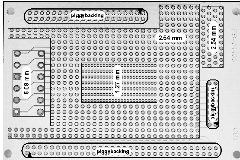
Figure 1: FLEX Thru Hole Daughter Board
